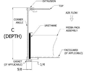
CROSS SECTION - SIDE VIEW
