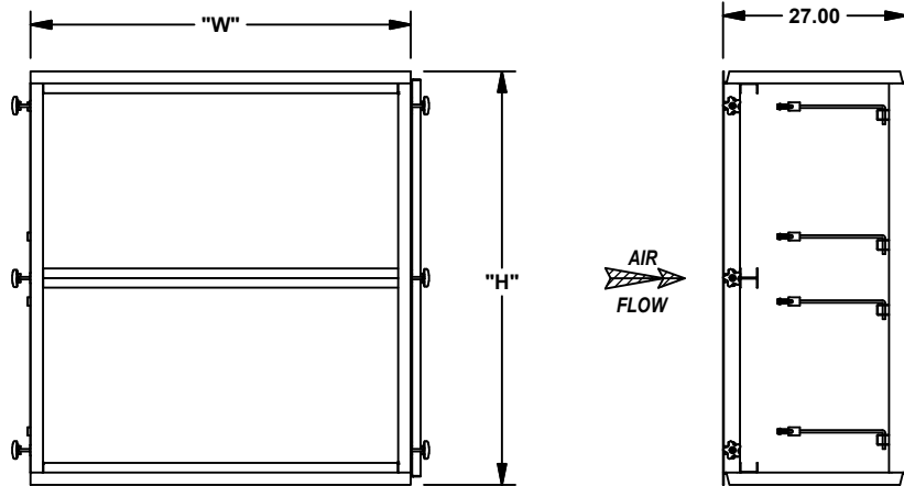
SIDE VIEW
