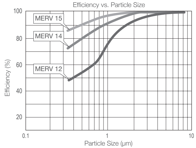
Composite Minimum Efficiency Curve
