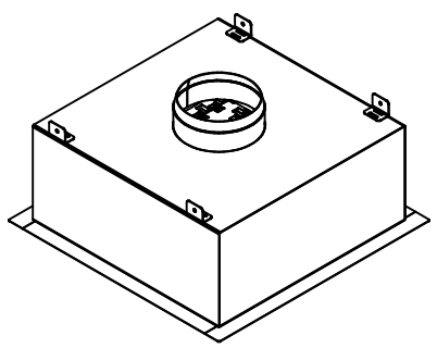
ISOMETRIC VIEW 1-1/2" [38.1mm] FIELD INSTALLED TRIM STYLE SHOWN
