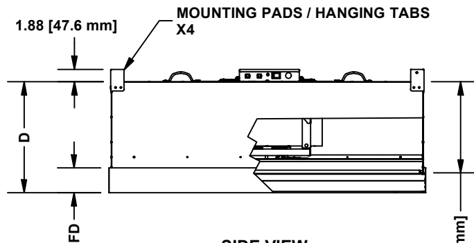
SIDE VIEW TOP SIDE SERVICEABLE SHOWN
